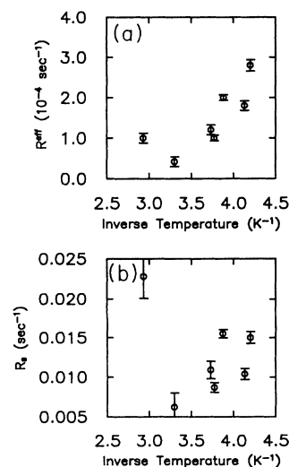
FIG. 10. (a) shows the measured value of the effective one-body bulk rate as a function of inverse temperature at B=7.62 T. (b) shows the surface rate extracted from the previous data according to Eq. (13).
